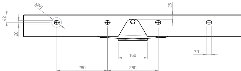
Backside view
